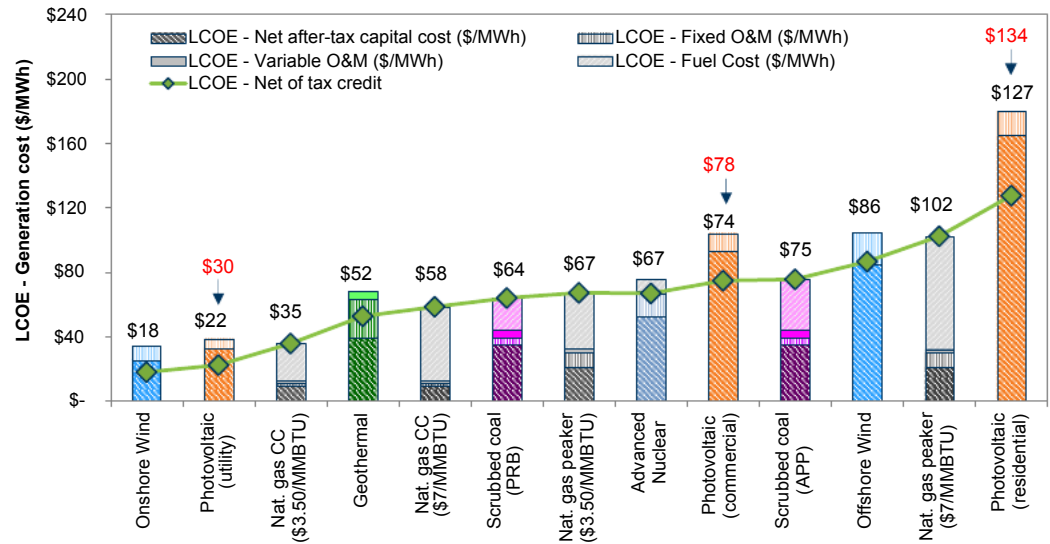
Exhibit 15: The reintroduction of the solar PTC would significantly reduce utility scale solar production costs
