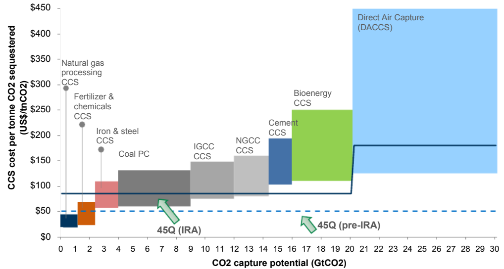
Exhibit 28: Global carbon capture cost curve and old/new US incentives for carbon capture with sequestration
