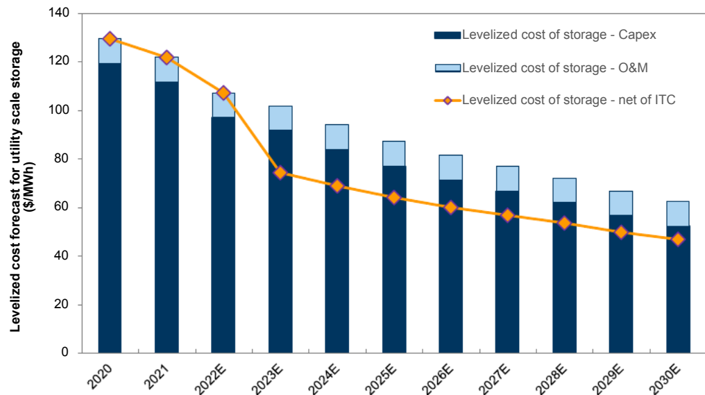
Exhibit 14: The levelized cost of utility-scale storage net of ITC in 2023 is expected to be 43% less than 2020, when there was no ITC for storage Innovation/cost deflation have also been contributing factors
